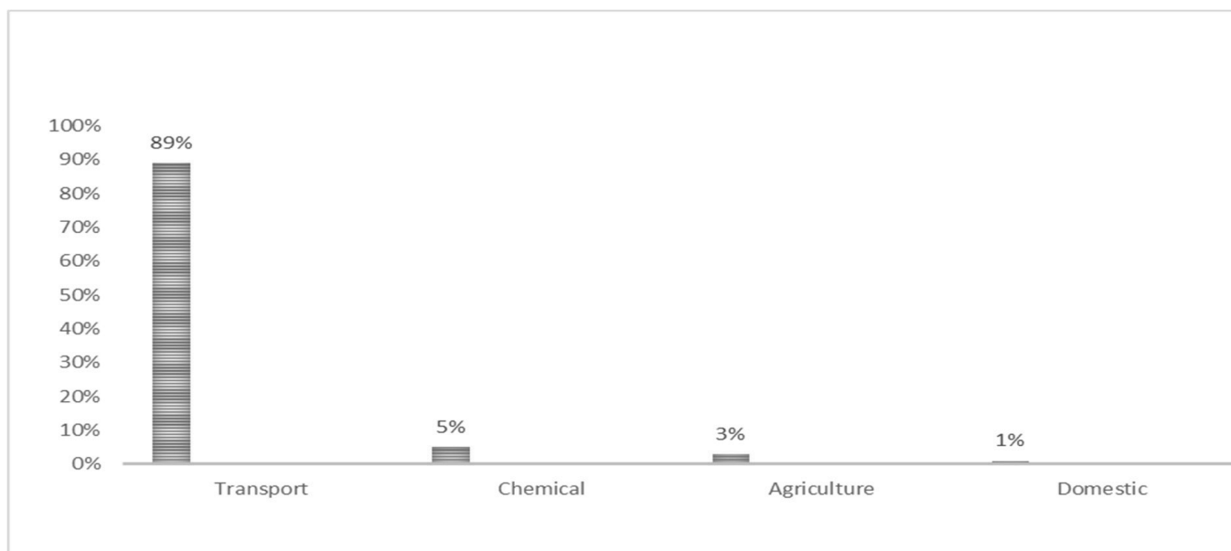
Figure 2: LPG consumption according to industry in Ukraine
